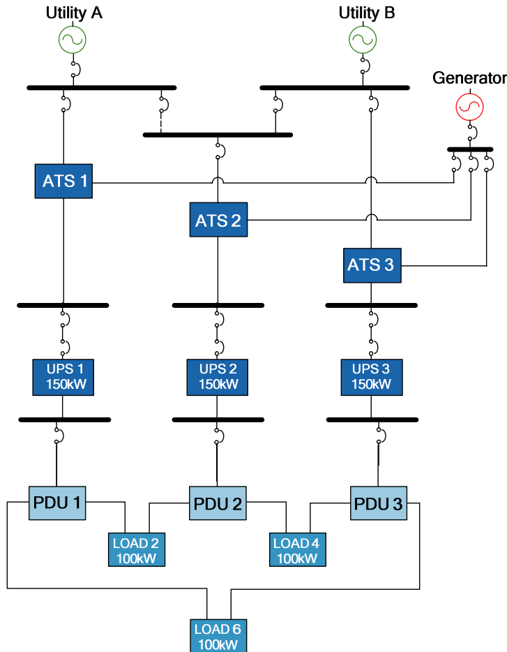
Figure 6 – Tri-redundant UPS configuration (no STS)
