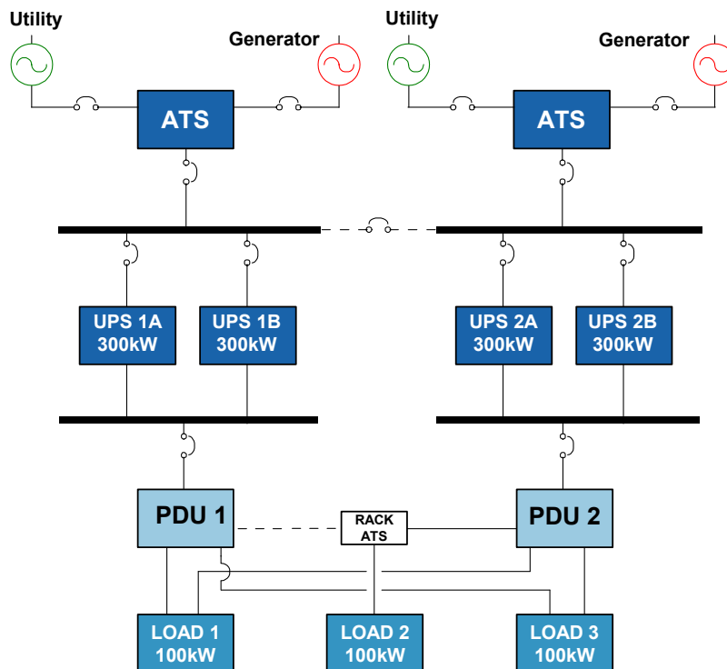
Figure 7 – 2(N+1) UPS configuration
