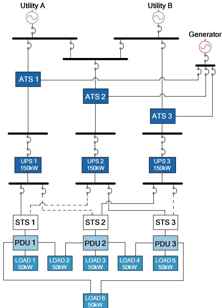
Figure 5 – Distributed redundant UPS configuration (with STS)
