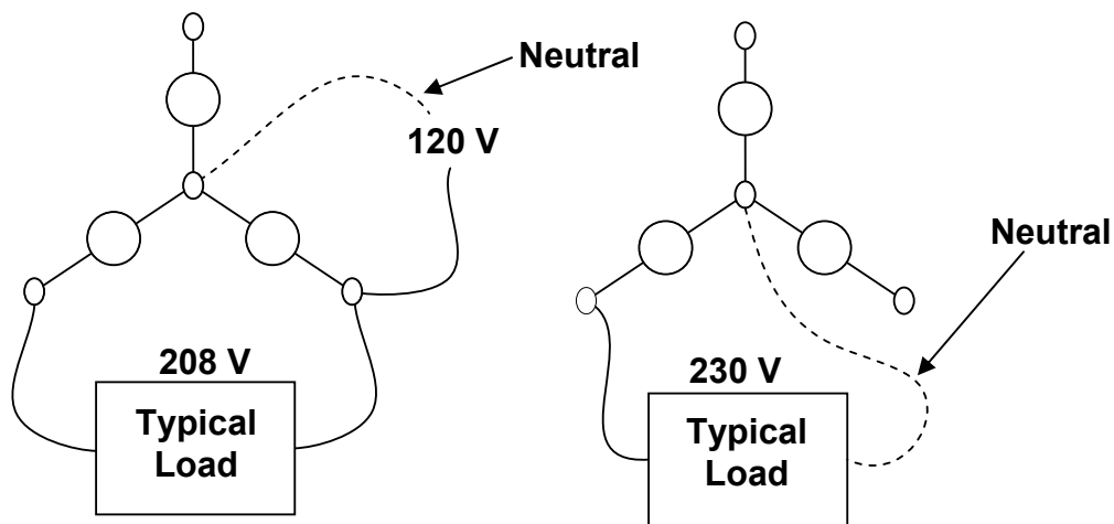
Figure 3 – Diagram showing the difference between three-phase 208 V distribution and 230 V distribution
