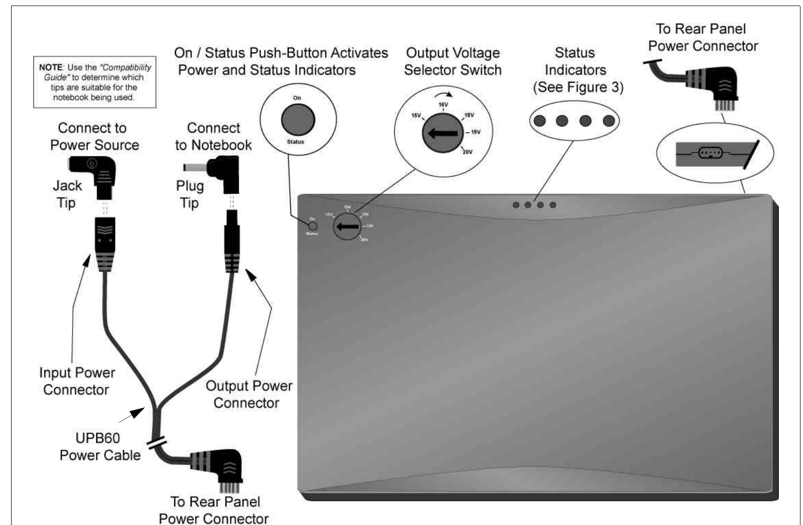
Figure 1. Universal Notebook Battery (UPB60) User Interface
